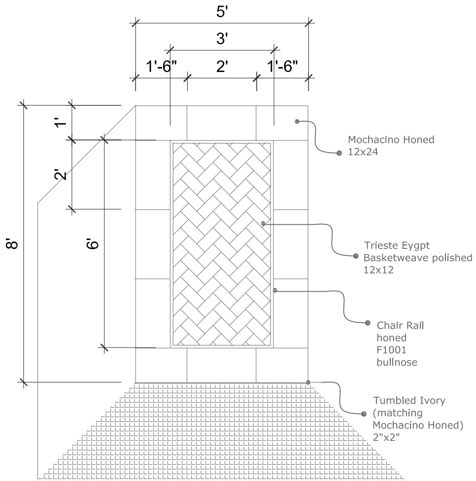
Roell Residence Master Ensuite Shower Tile Layout 5'-0" back wall
